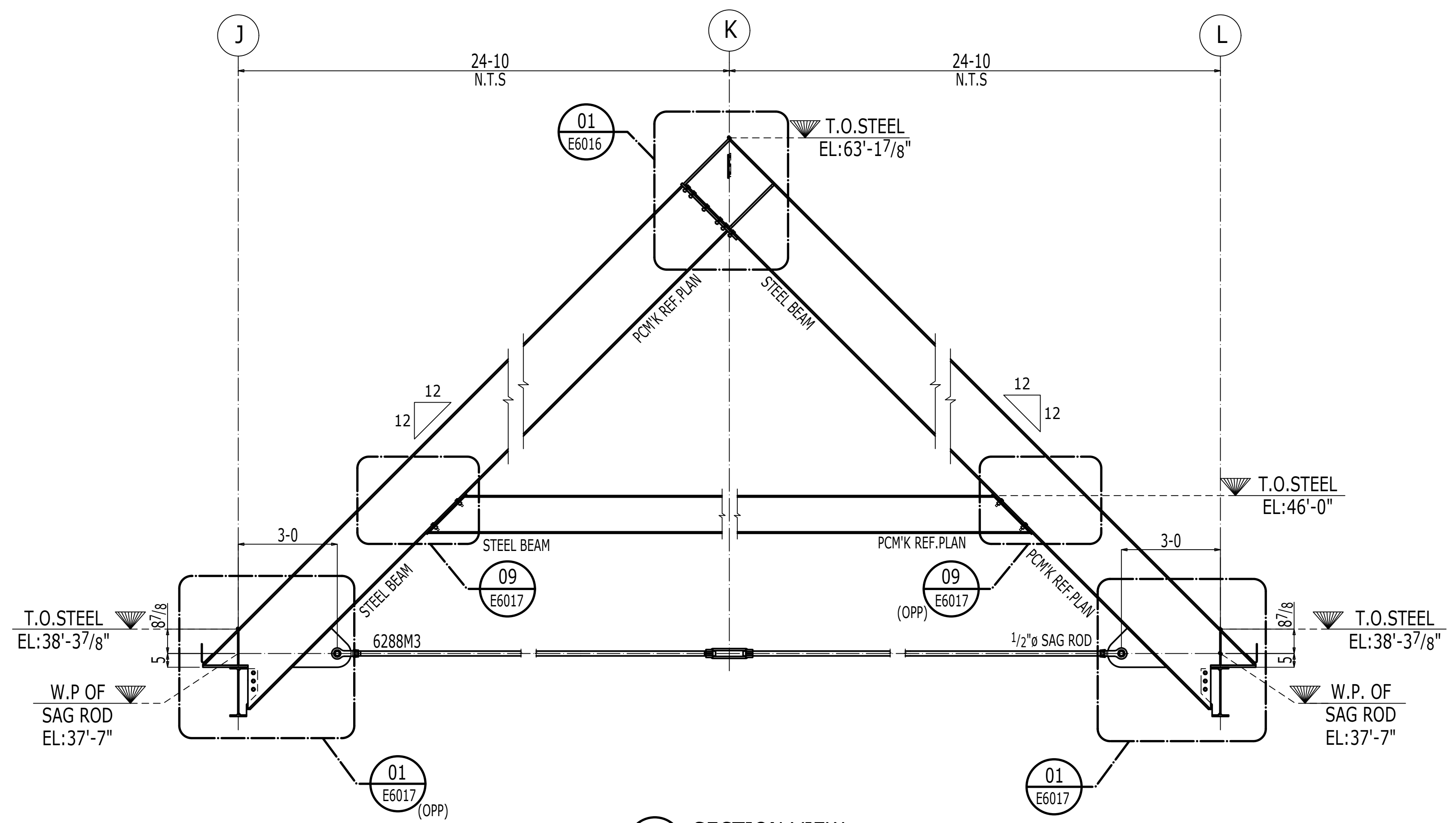
03 SECTION VIEW E6010
