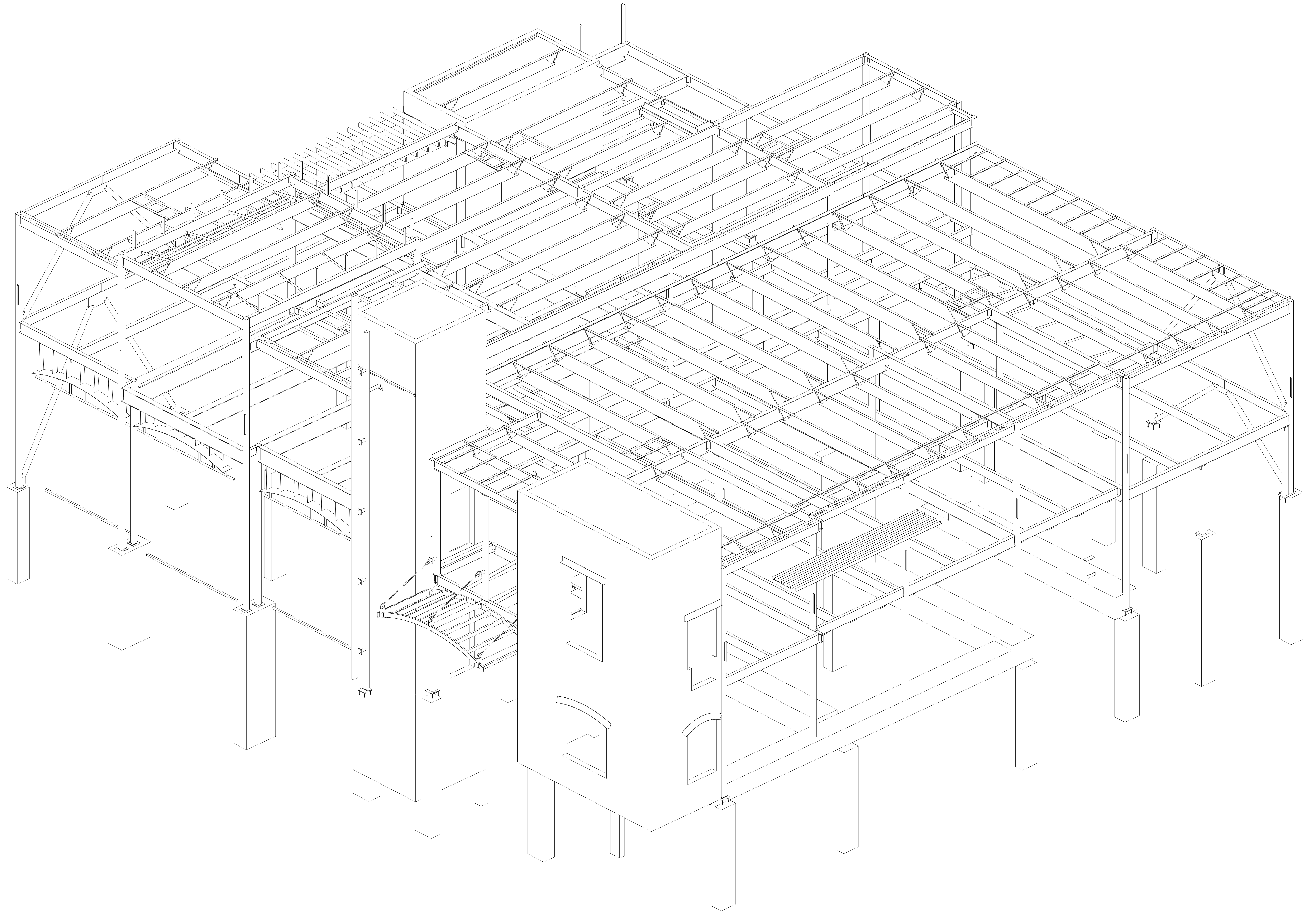
ISOMETRIC VIEW
